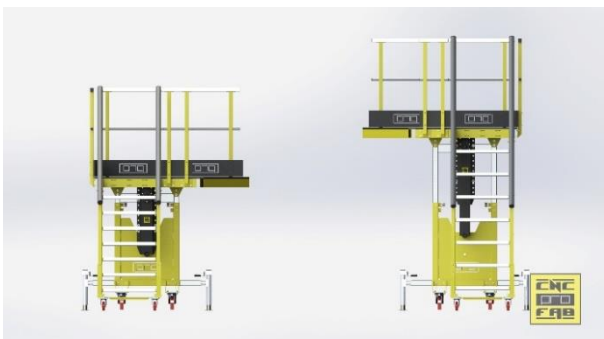
700mm HEIGHT ADJUSTMENT
